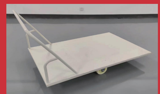
Cloth transport trolley (布匹运输车) Size:L1600*W1000*H760mm
