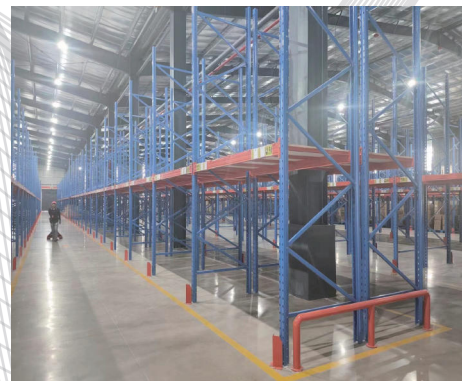
Finished product racks (一层横梁成品货架) Size:L2500*W1000*H4500mm
