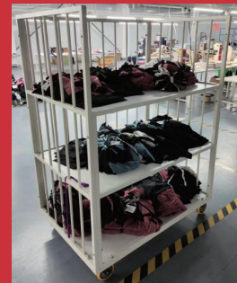
Three layers round tube cut pieces trolley (三层圆管裁片车) Size:L1200*W800*H1600mm
