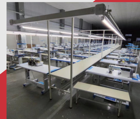
Sewing line center table with light (灯杆式流水线案板)
